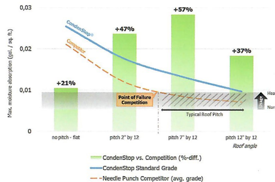
Absorption Performance: CondenStop® vs. Generic Needle Punch Moisture absorption by roof pitch angle - Absolute & relative performance
